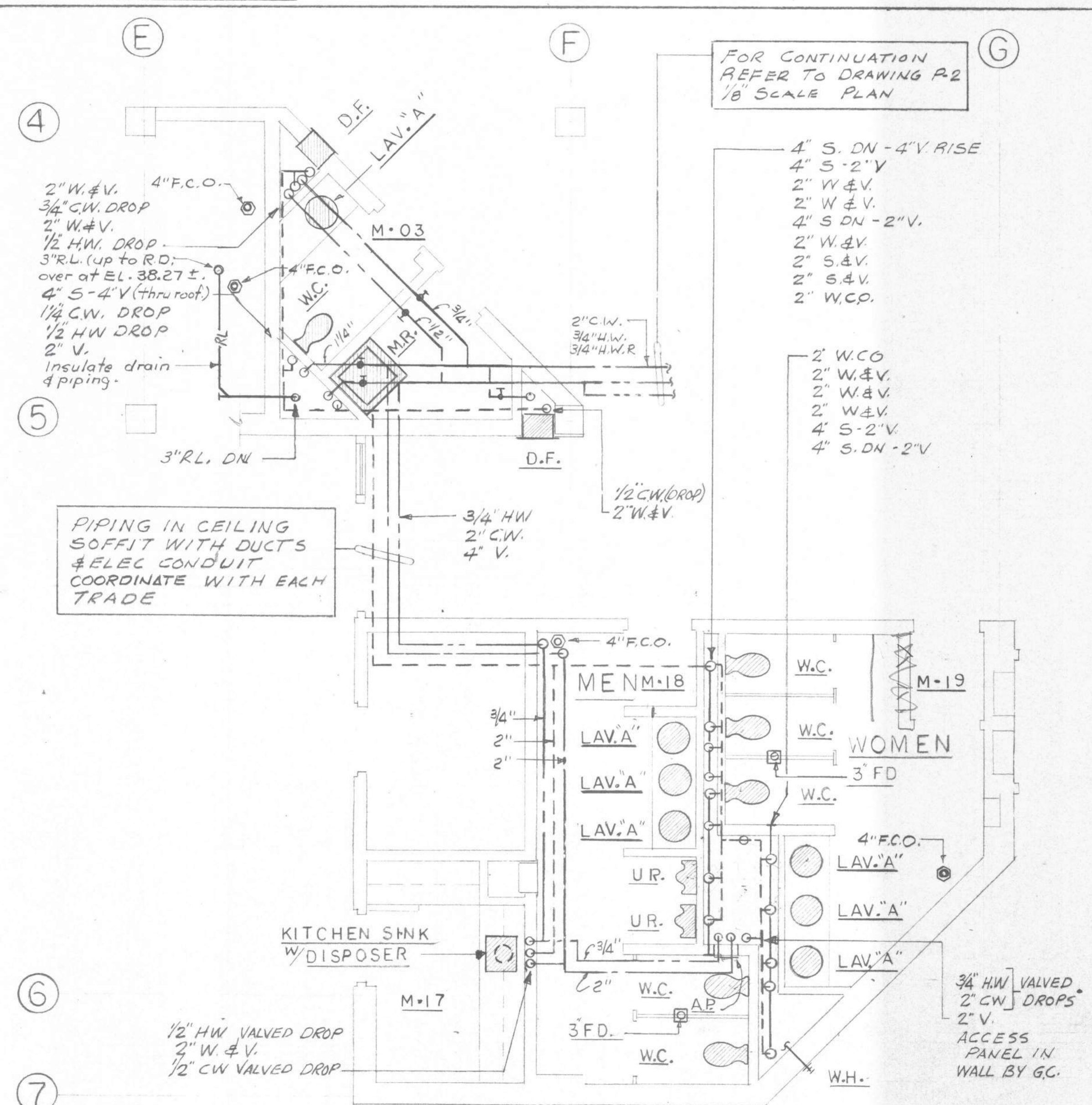
ENLARGED PLAN OF TOILET ROOMS SCALE 1/4"=1'-0"
