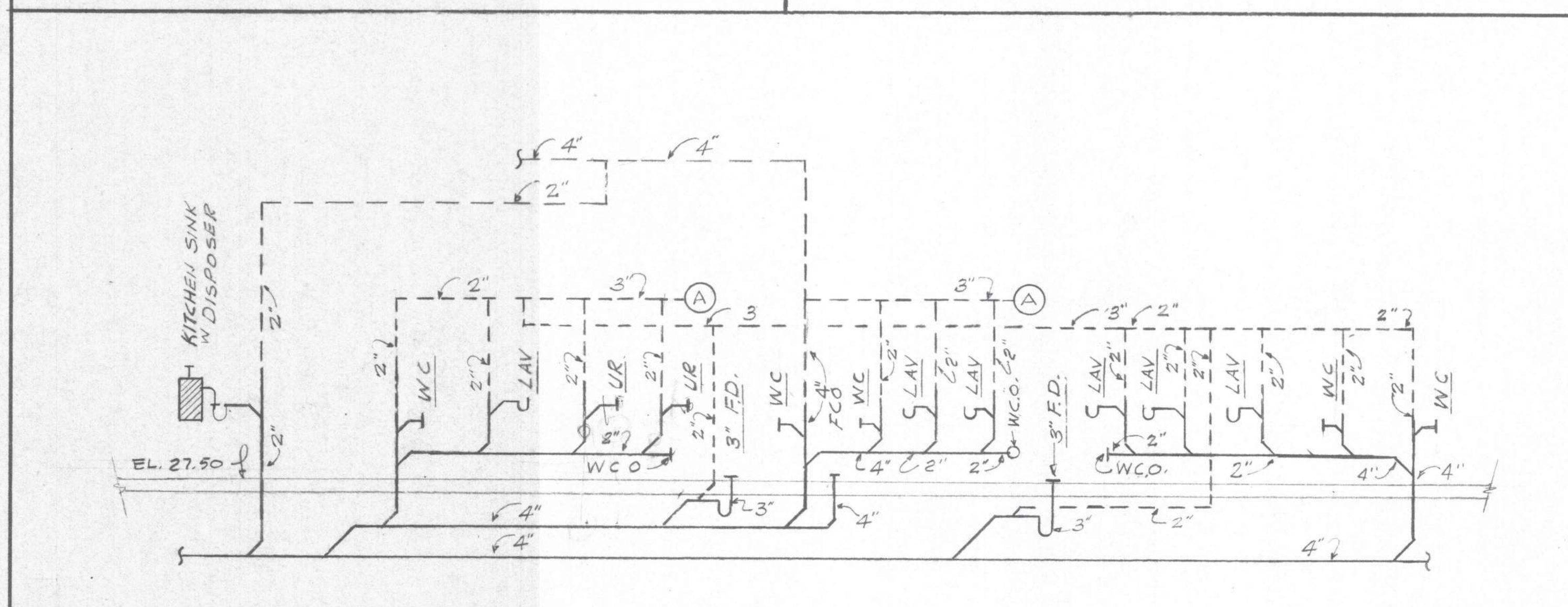
PART SOIL WASTE VENT PIPING DIAGRAM NO SCALE
