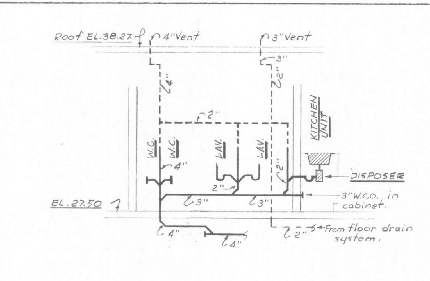
STAFF TOILET R.M.'S. & KIT. UNIT PIPING DIAGRAM NO SCALE
