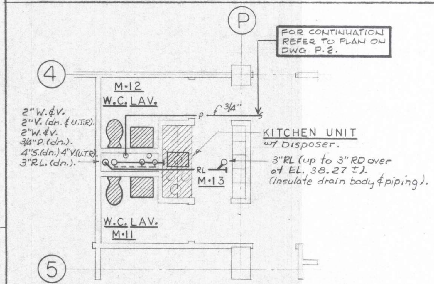
STAFF TOILET R.M.'S. & KIT. UNIT SCALE: 1/4"=1'-0"
